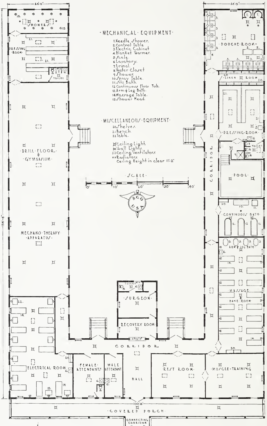
⑤ PHYSICAL THERAPY BUILDING
